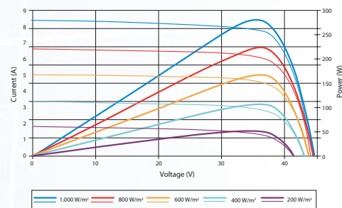
Current-Voltage & Power-Voltage Curve (280-24)
